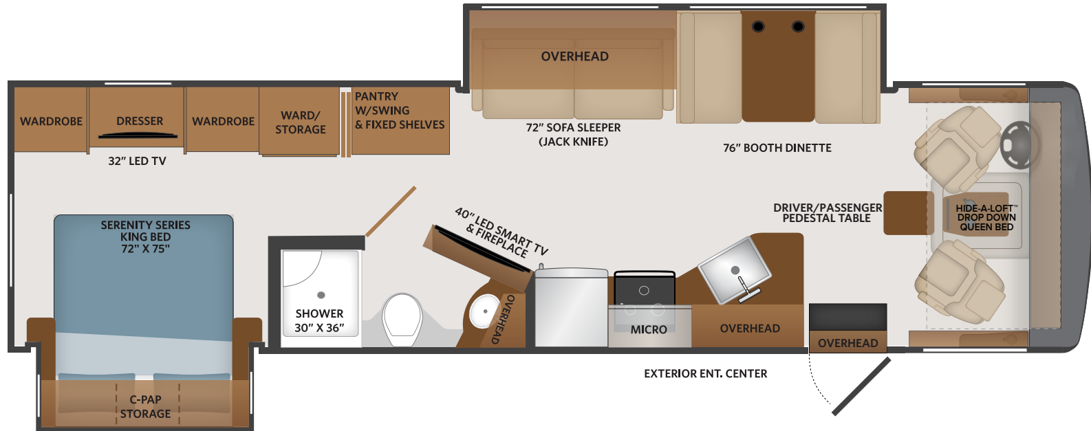
OPT. 131 WASHER & DRYER STACKABLE
