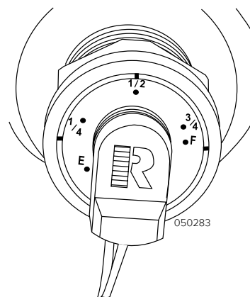
Gauge Mounted on Propane Tank
