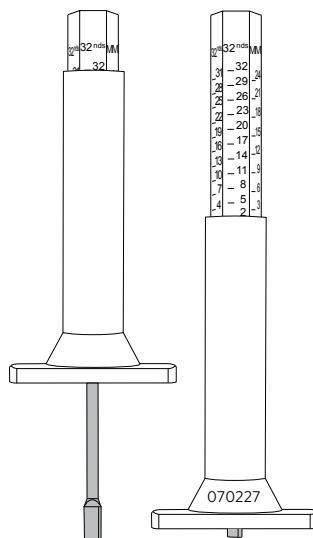
Tire Groove Depth Gauge
