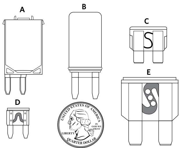
Representation of various fuses and a circuit breaker. 080528e
