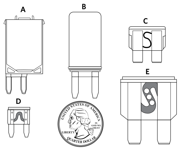
Representation of various fuses and a circuit breaker. 080528e Quarter is used for size comparison of fuses. A. Manual Reset Circuit Breaker B. Auto Reset Circuit Breaker C. Standard Fuse D. Mini Fuse E. Maxi Fuse
