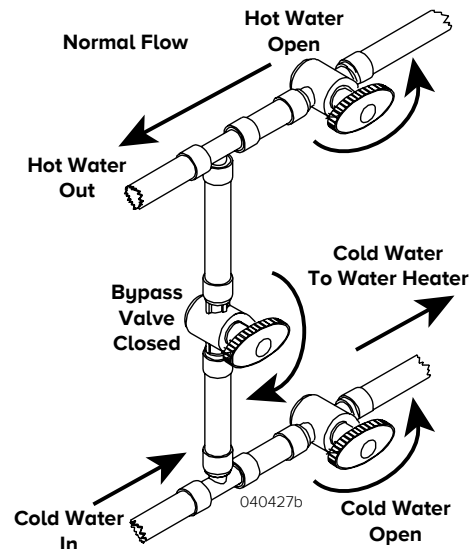
Bypass Valves Located Behind Water Heater
