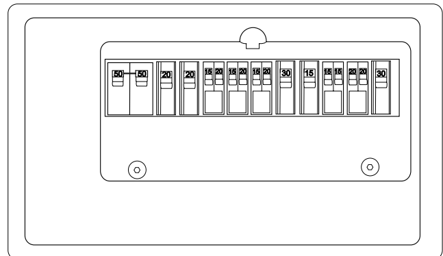
Load Center Located Above Pilot Seat
