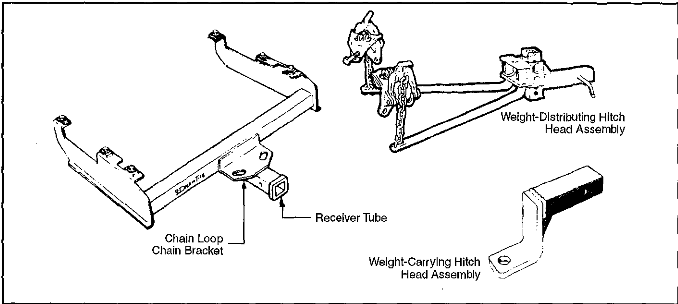
Typical Hitch System Components
