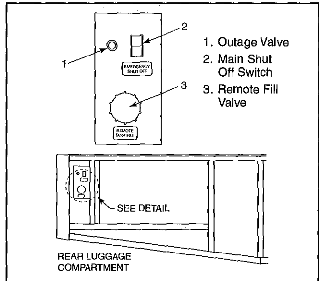
Remote LP Gas Tank Fill
