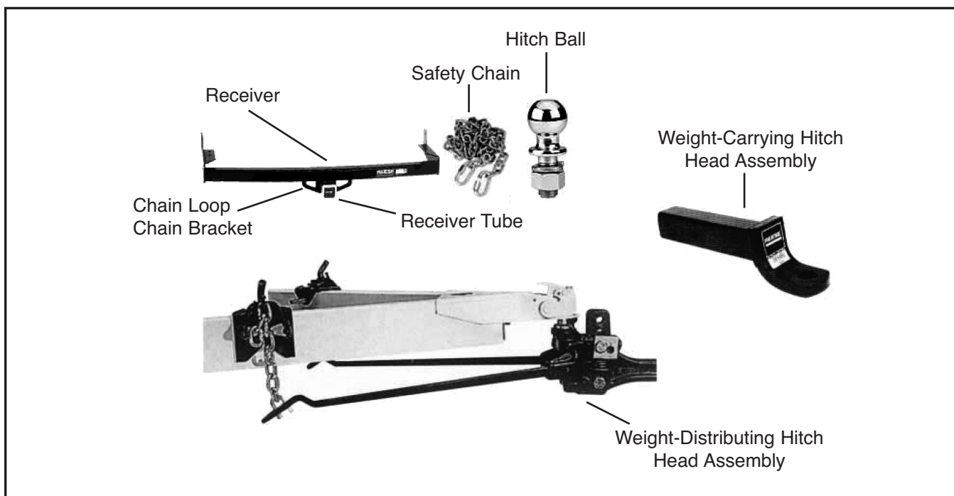
Typical Hitch System Components
