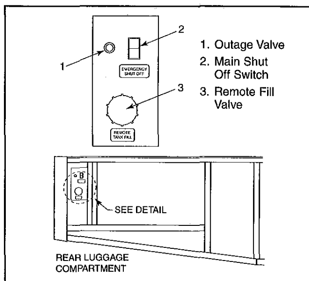
Remote LP Gas Tank Fill
