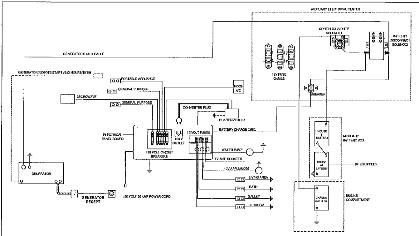
Typical Electrical Diagram
