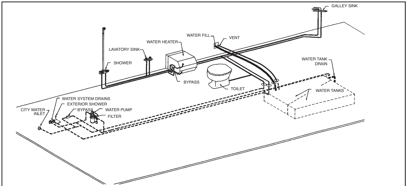
Typical Hot and Cold Diagram (Note: This is a "typical" plumbing installation. There may be variations due to your particular model and installed options).
