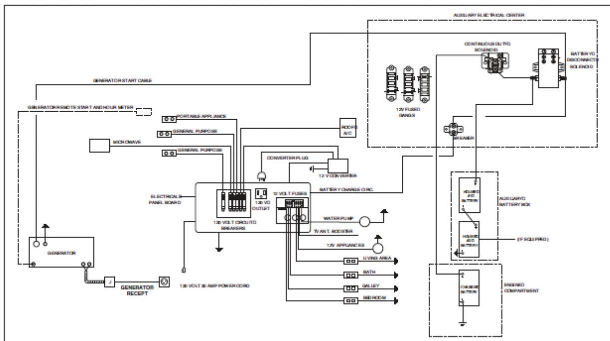
Typical Electrical Diagram
