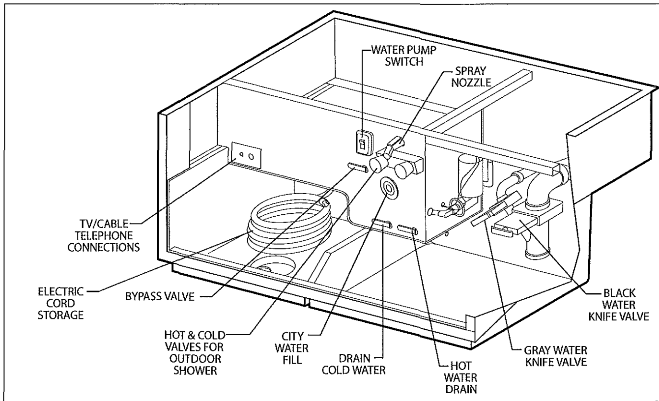
Utility Compartment (detail varies depending on product)
