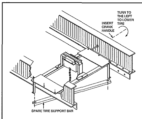
Spare Tire Carrier
