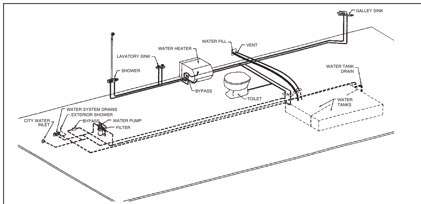
Typical Hot and Cold Diagram (Note: This is a “typical” plumbing installation. There may be variations due to your particular model).
