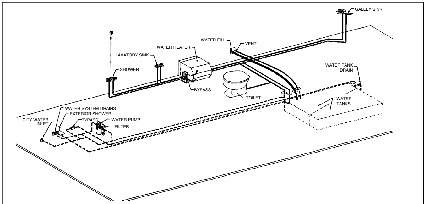
Typical Hot and Cold Diagram (Note: This is a “typical” plumbing installation. There may be variations due to your particular model).
