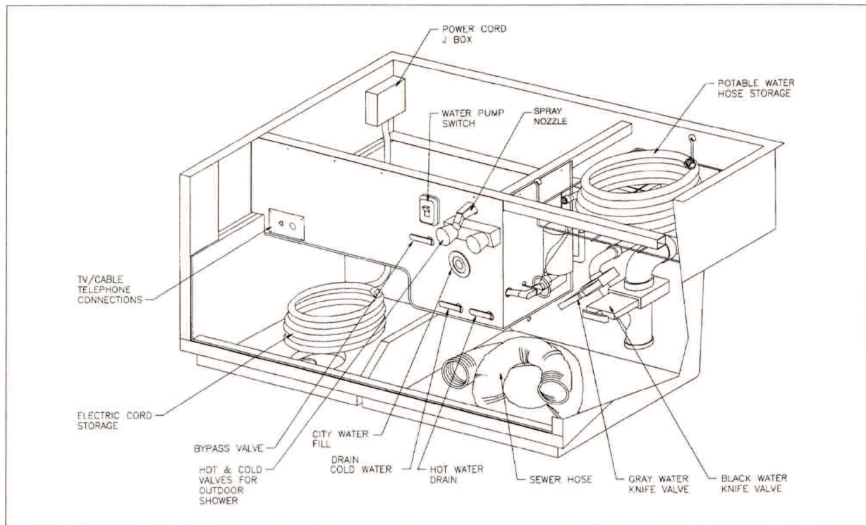
Utility Compartment (detail varies depending on product)
