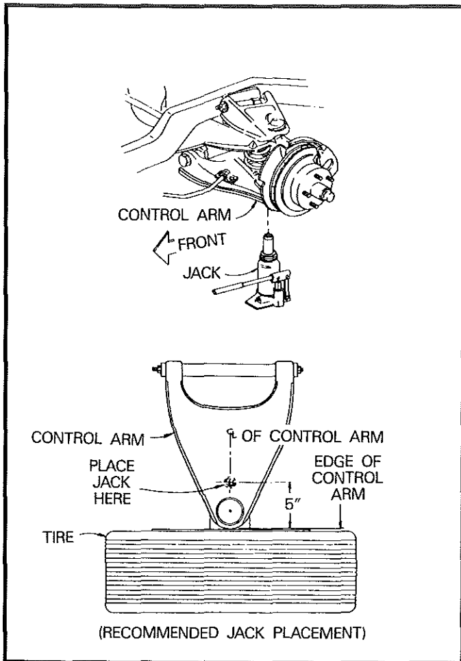
Jack Position — Front Chevrolet Chassis
