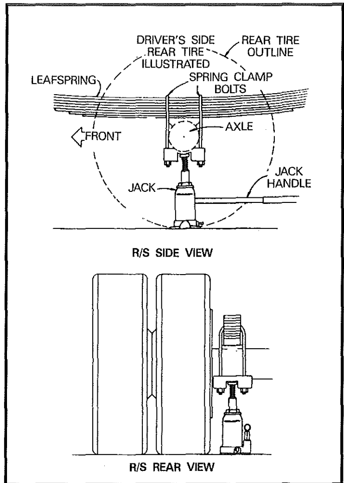
Jack Position — Rear Chevrolet Chassis
