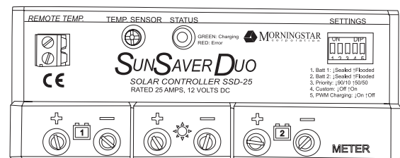
Charge Controller
