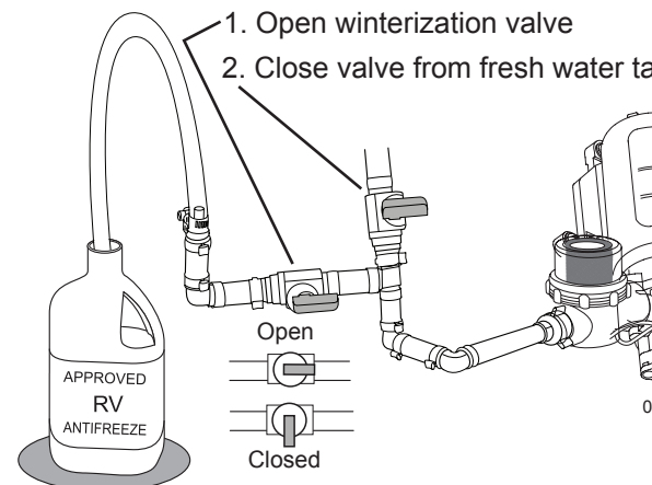
Winterization procedure using non-toxic antifreeze
