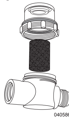
Water pump inlet screen: Clean every two months.
