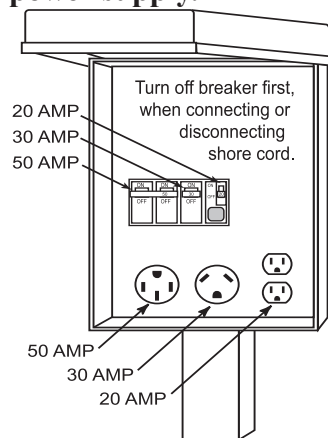
Typical power pedestal
