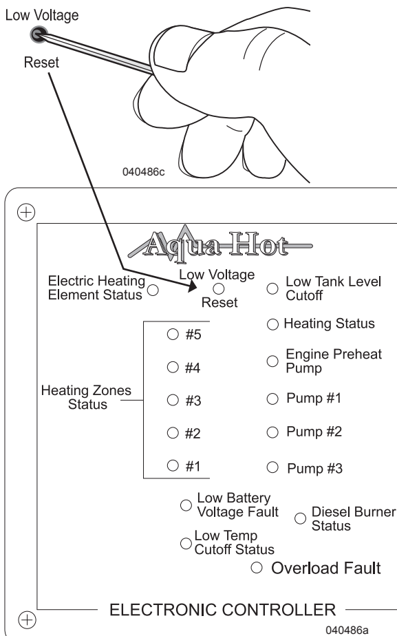
Electronic controller located in Aqua-Hot
