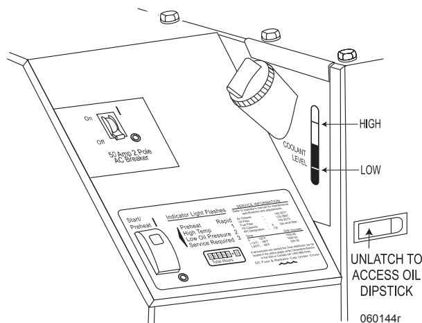
Coolant level window
