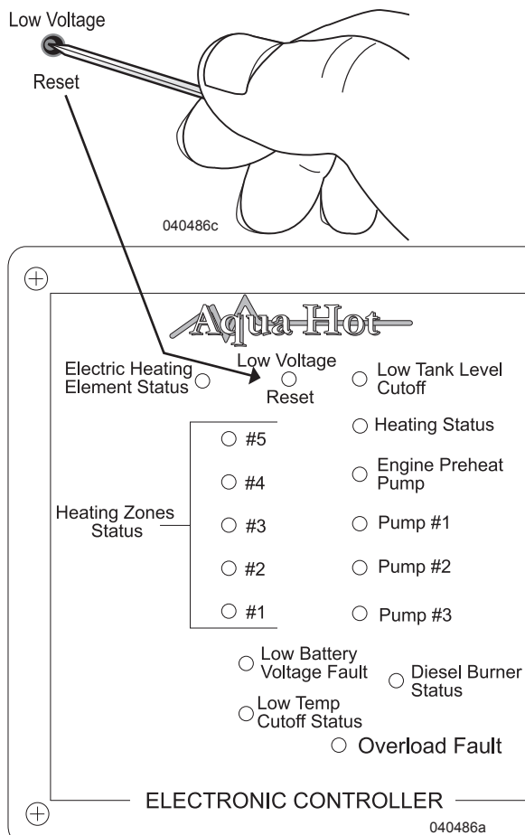
Electronic controller located in Aqua-Hot
