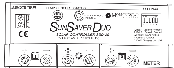
Charge Controller
