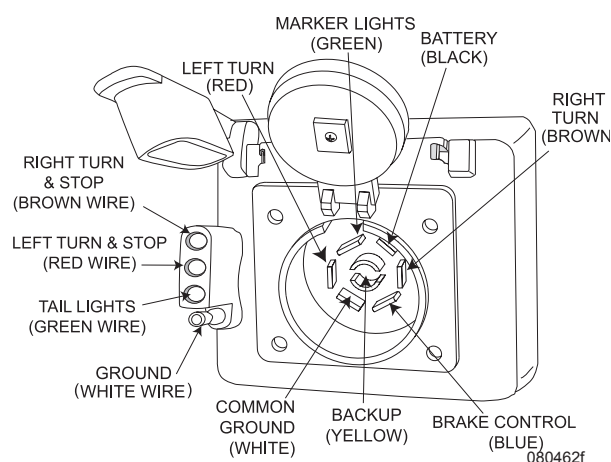
Tow plug index
