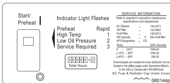
Panel located on generator
