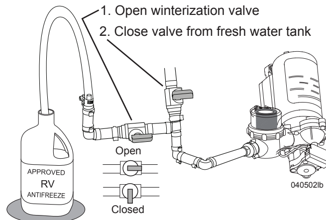
Winterization procedure using non-toxic antifreeze
