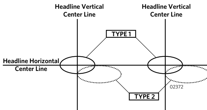
Headlamp Adjustment
