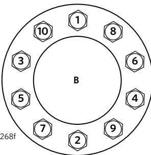
Lugnut Torque Sequence
