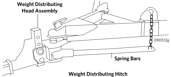
Weight Distributing Hitch
