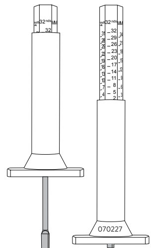
Tire Groove Depth Gauge
