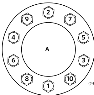
Lugnut Torque Sequence
