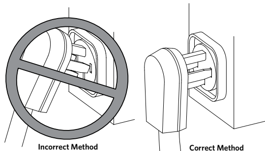
30 amp Outlet Shown
