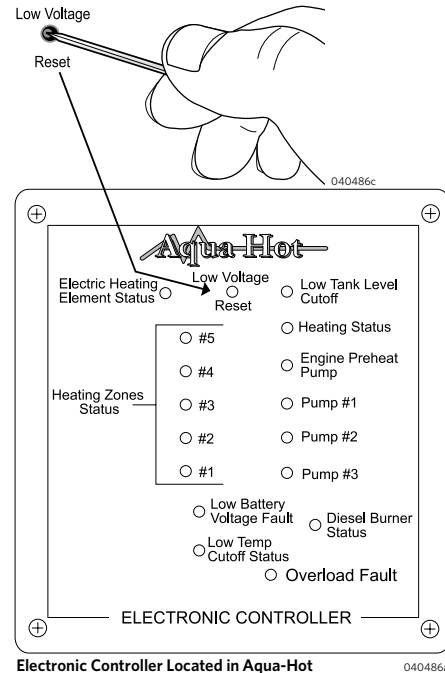
Electronic Controller Located in Aqua-Hot
