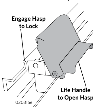
Egress Style A (shown in unlocked position)
