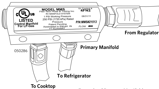
Example of Propane Manifold
