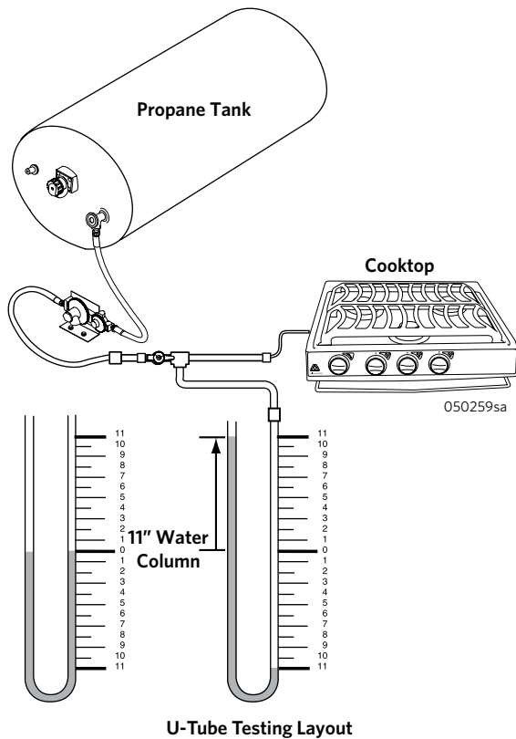
U-Tube Testing Layout
