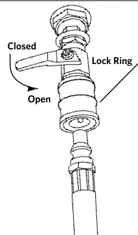
Barbecue Quick Disconnect
