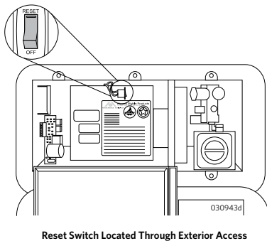
Reset Switch Located Through Exterior Access
