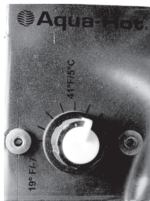
Aqua-Hot Thermostat (located behind service panel) It is factory preset and should not require adjustment.
