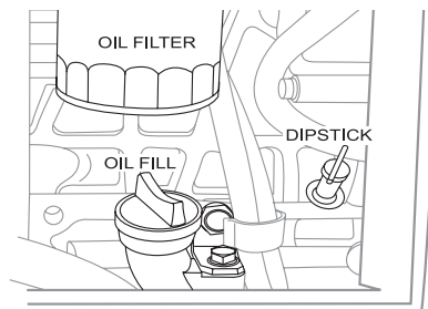
10 Kw Oil Dipstick Located Behind Access Door On Generator
