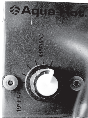
Aqua-Hot Thermostat (located behind service panel) It is factory preset and should
