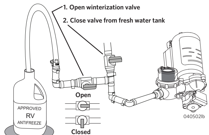
Winterization Procedure Using Non-Toxic Antifreeze
